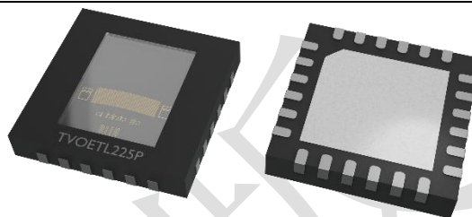
QFN32 5.0 mm × 5.0 mm × 0.9 mm RoHS
