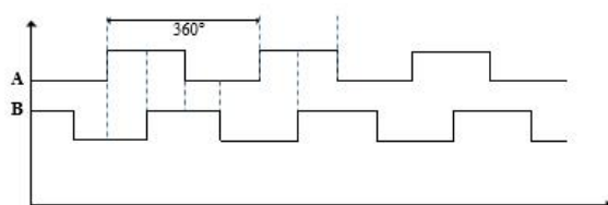
Figure: Sample of Output Waveforms
